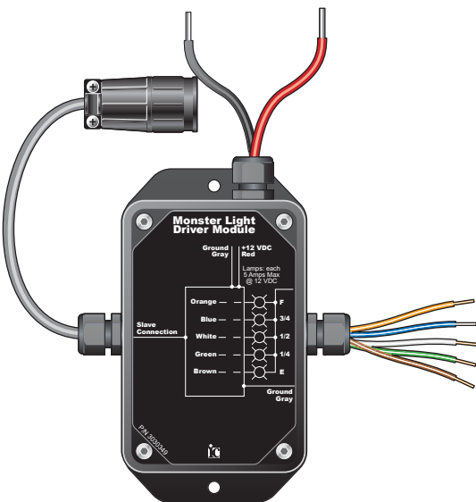
IC P/N 3030349 LC / XP Series Monster Light Relay Driver Module
