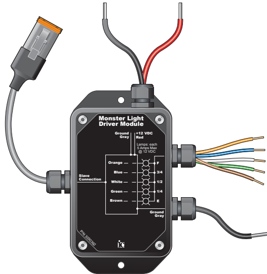
IC P/N 3030362 SL Series Monster Light Relay Driver Module
