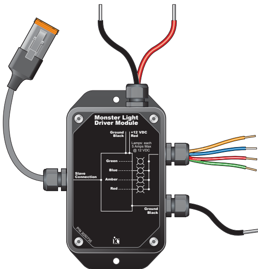
IC P/N 3030735 SL Plus Monster Light Relay Driver Module (for use with alternative monster lights)
